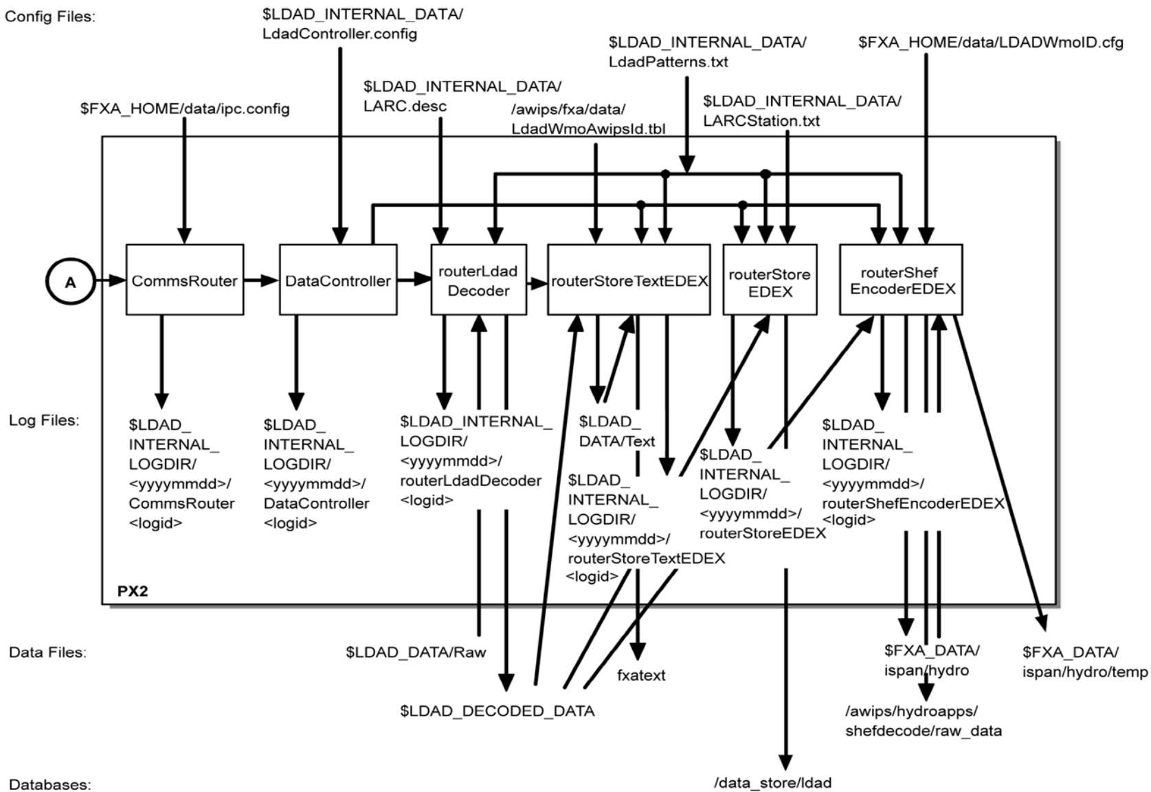
Exhibit 8.3.1-1. Generic Acquire and Decode LDAD Product (Page 2 of 2)
