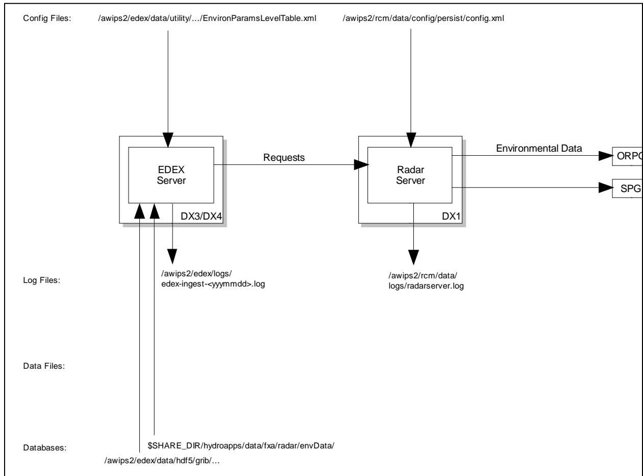
Exhibit 7.6-1. Sending Environmental Data
