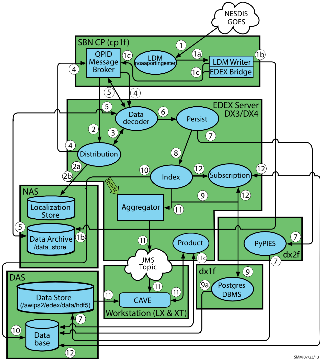
Exhibit 6.2-1. NWSSTG (grib and non-grib) Data Flow
