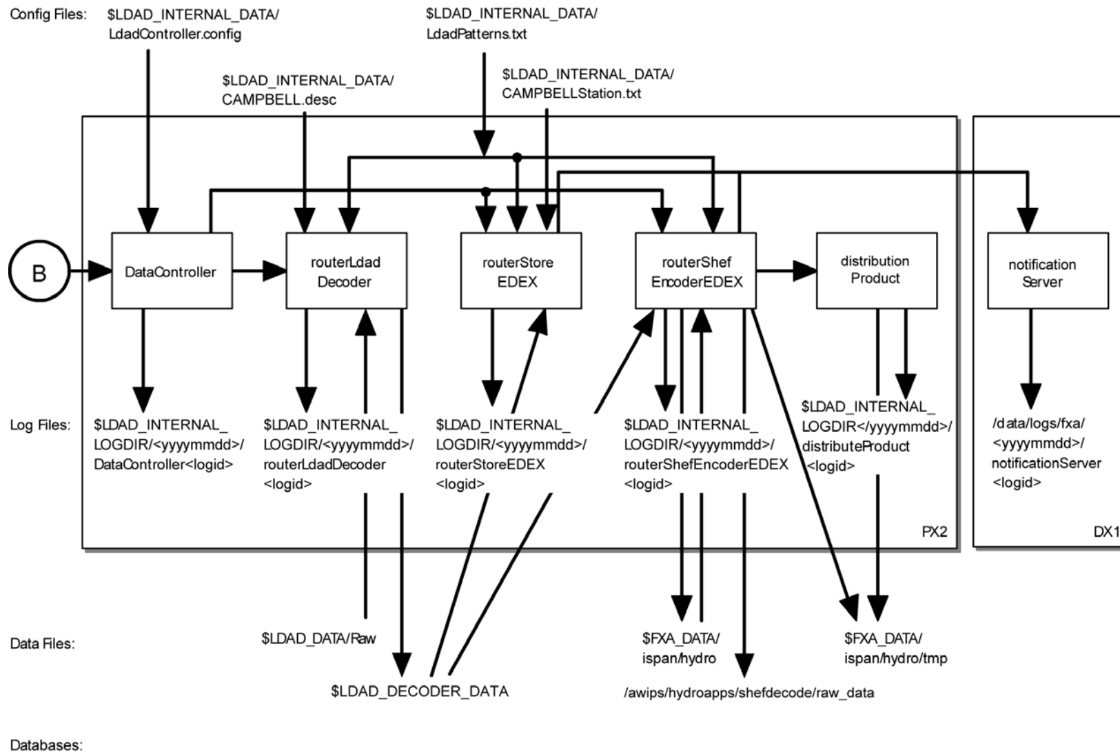
Exhibit 8.10-1. Decode Campbell Data (for LDAD) (Page 2 of 2)
