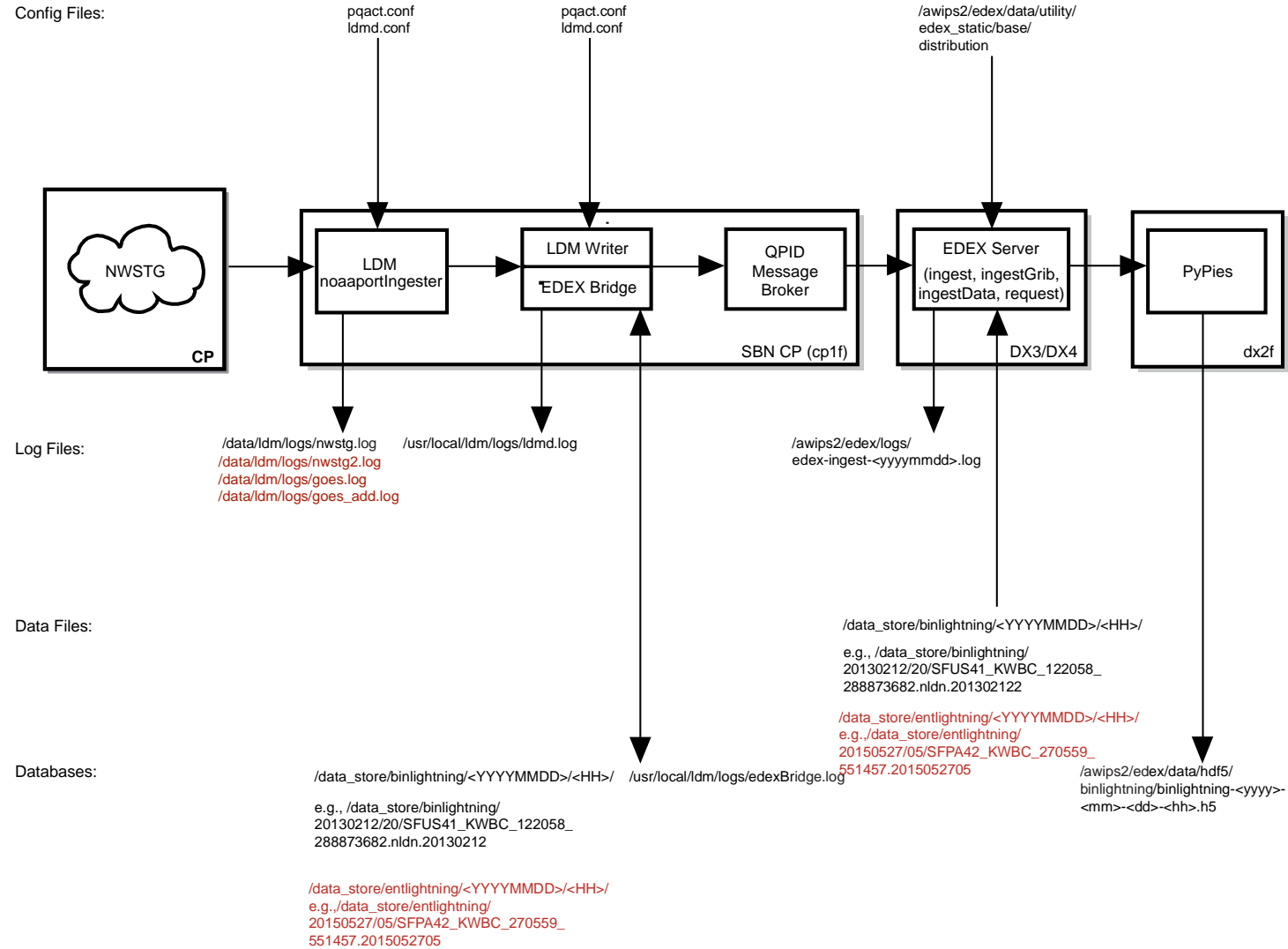
Exhibit 6.3-1. Acquire and Ingest of Lightning Products
